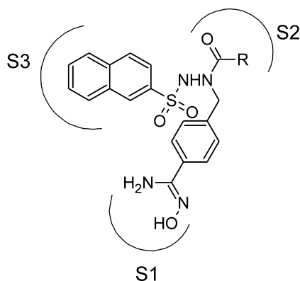
Figure 2. Schematic drawing of the thrombin inhibitor in the active site of thrombin (R moieties are defined in Table 4).
