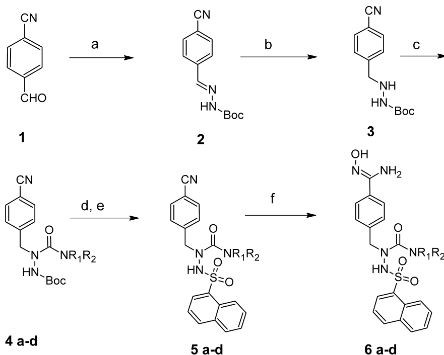
Scheme 1. (a) Boc-NHNH 2 , EtOH, reflux, 95%; (b) H 2 , Pd/C, MeOH, 97%; (c) (1) (Cl 3 CO) 2 CO, CH 2 Cl 2 , (2) HNR 1 R 2 , DIEA, 35–81%; (d) HCl (g), AcOH; (e) naphthalene-2-sulfonyl chloride, CH 2 Cl 2 , Et 3 N, 22–33%; (f) NH 2 OH, EtOH, reflux, 38–57%.
