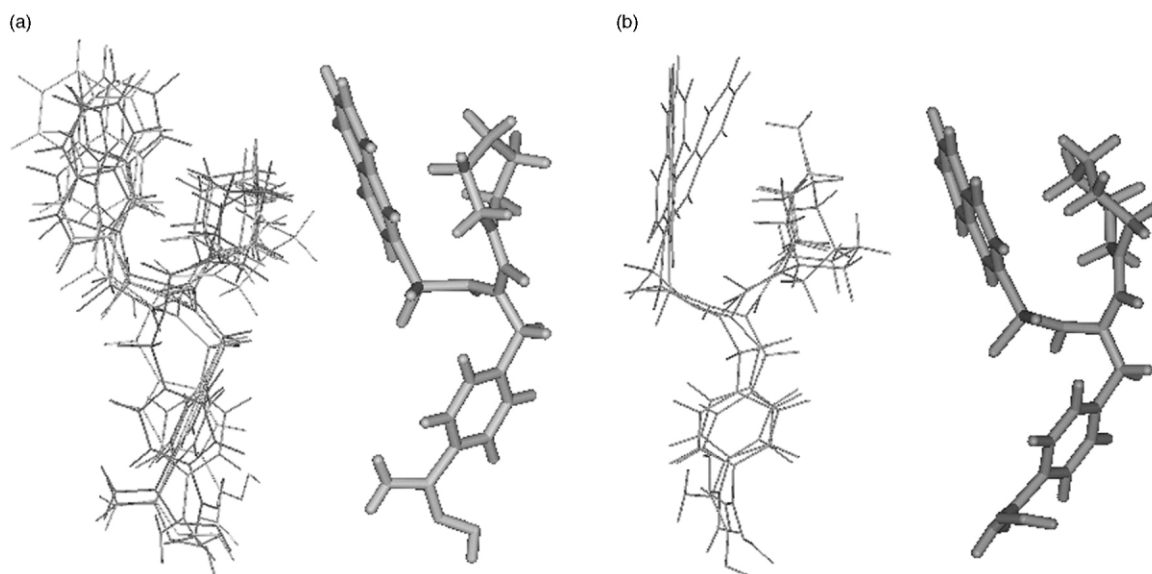
Figure 3. (a) Comparison of solution conformations of 6a (thin lines) with the conformation of 6a (heavy lines) as modeled in the thrombin active site. The various orientations of the naphthalene, piperidine ring and benzamidoxime are shown. (b) Comparison of solution conformations of 6b-c (thin lines) with the structure of 6a (heavy lines). The various orientations of the naphthalene, piperidine and benzamidoxime moiety are shown.
