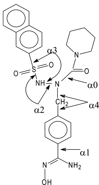
Figure 4. Torsion angles definitions in molecules 6a–d .
