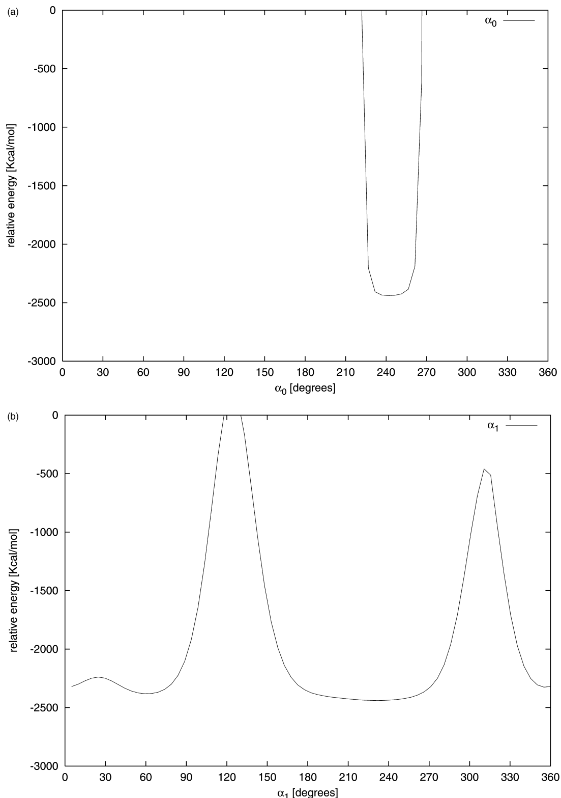
Figure 5. (a) Relative energy profiles for conformational dependence of the inhibitor–thrombin complex on \alpha_0 . (b) Relative energy profiles for conformational dependence of the inhibitor–thrombin complex on \alpha_1 .
