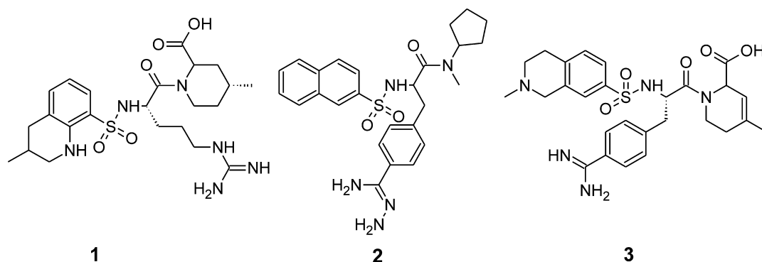
Figure 1. Structures of thrombin inhibitors.
